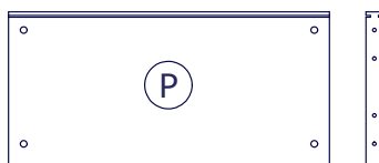
• PI6231 722x351x38mm
