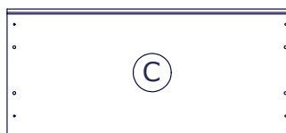
• CA2863 800x356x38mm
