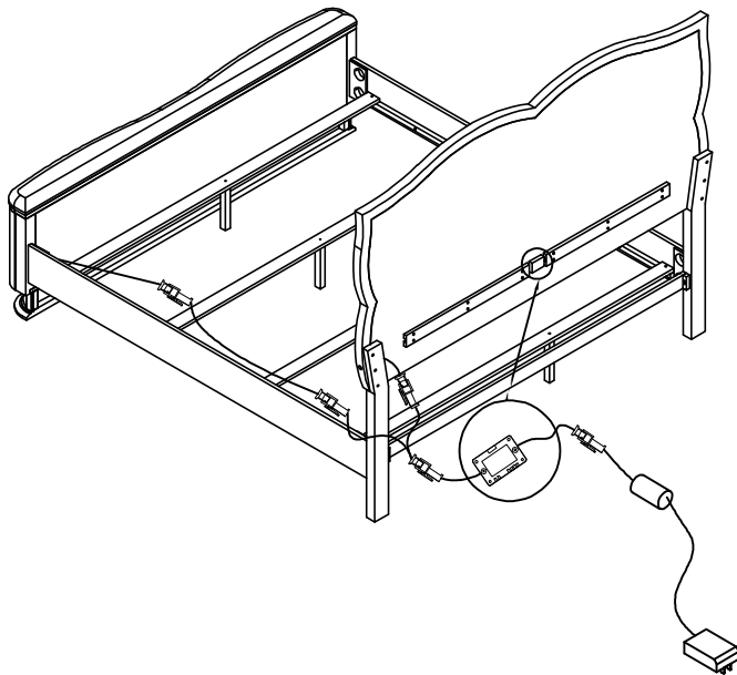
ELECTRICAL CONNECTION DIAGRAM.
