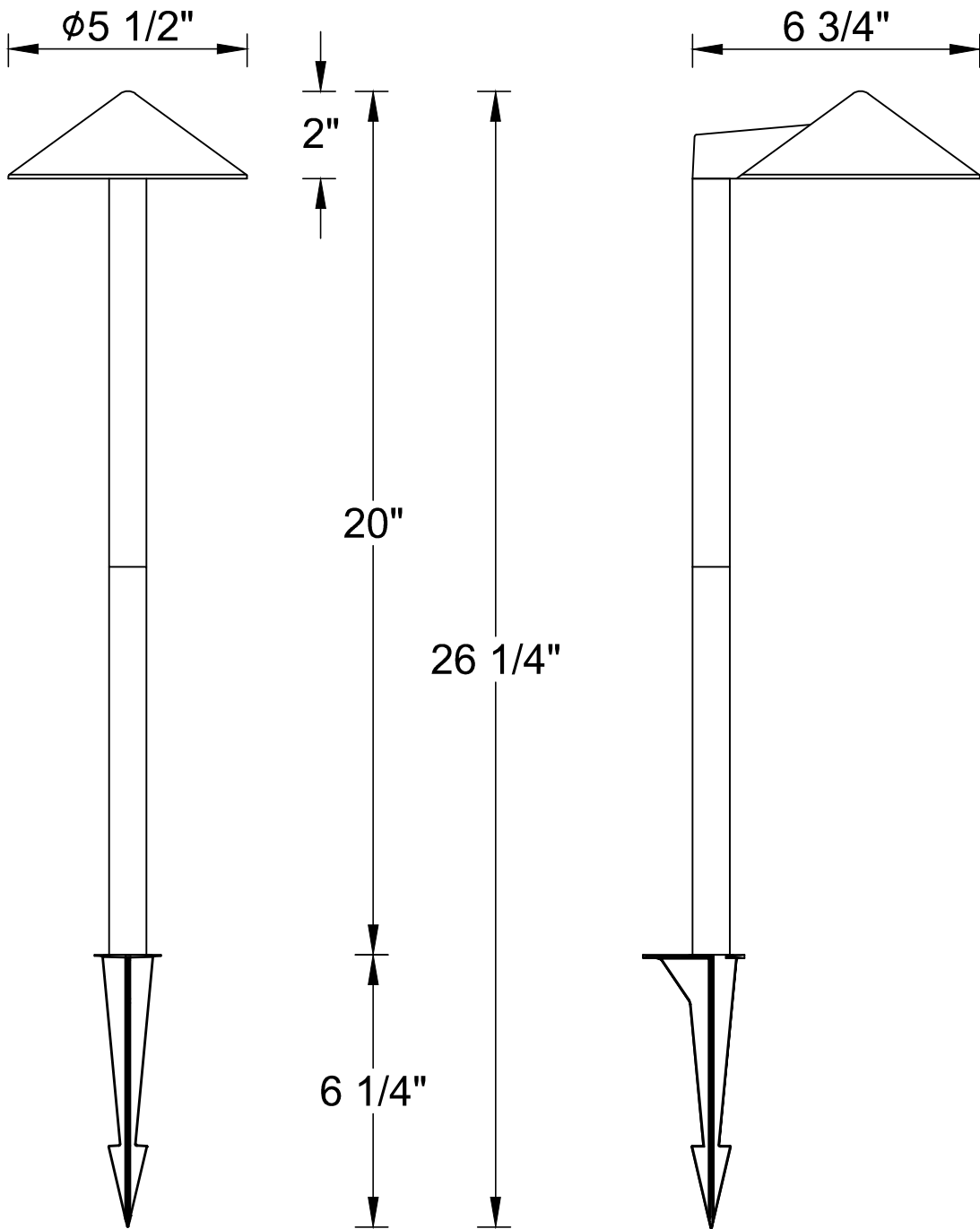
FRONT VIEW
