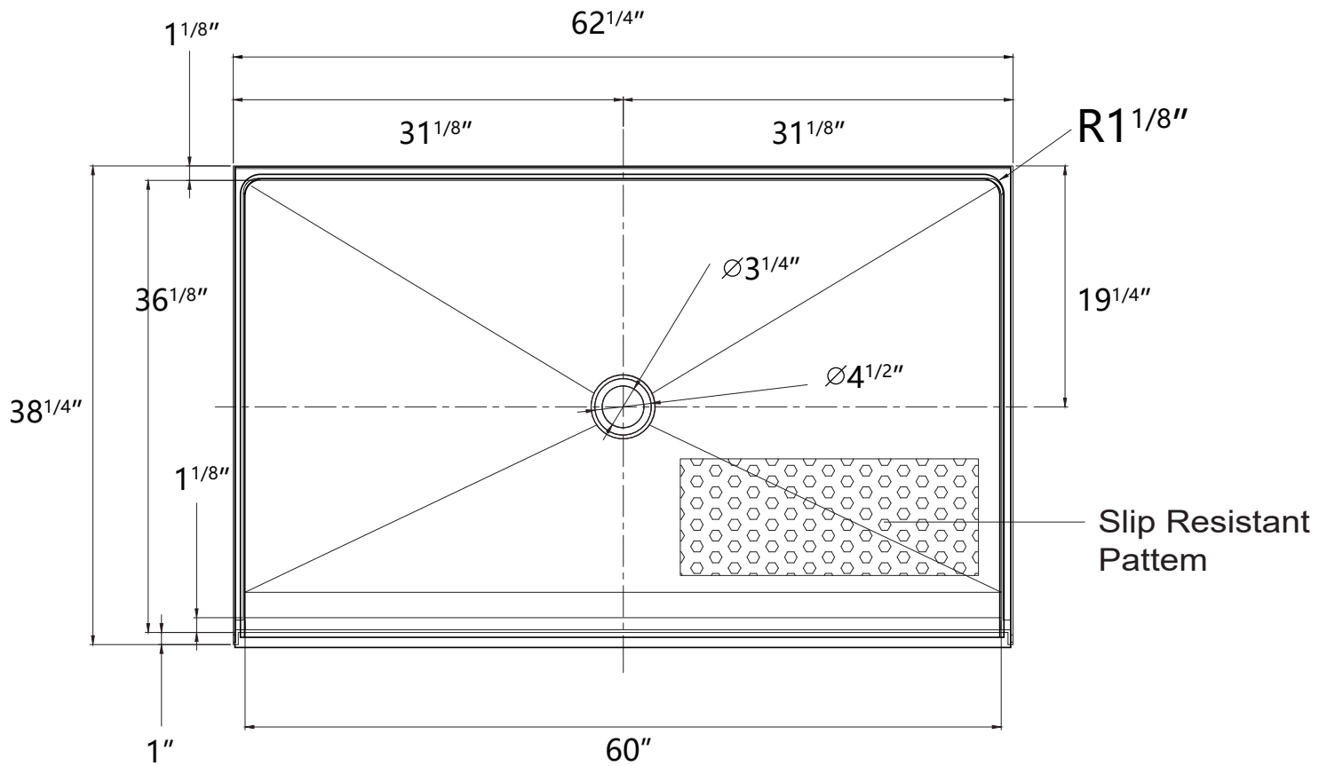
Top View
