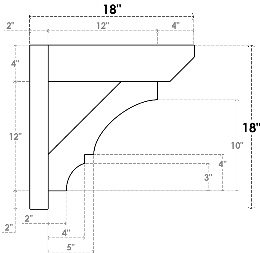
SIDE PROFILE
