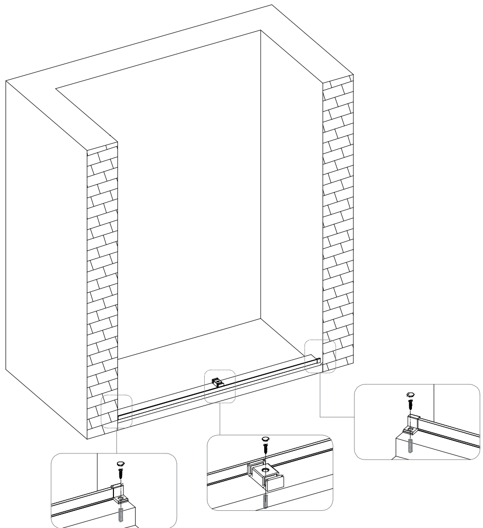
Lower Water Stop Bar Fixing Parts
