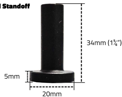
NT.1303-34mm.08 (For doors up to 1 1/2" thick)
