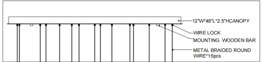
CANOPY DETAIL
