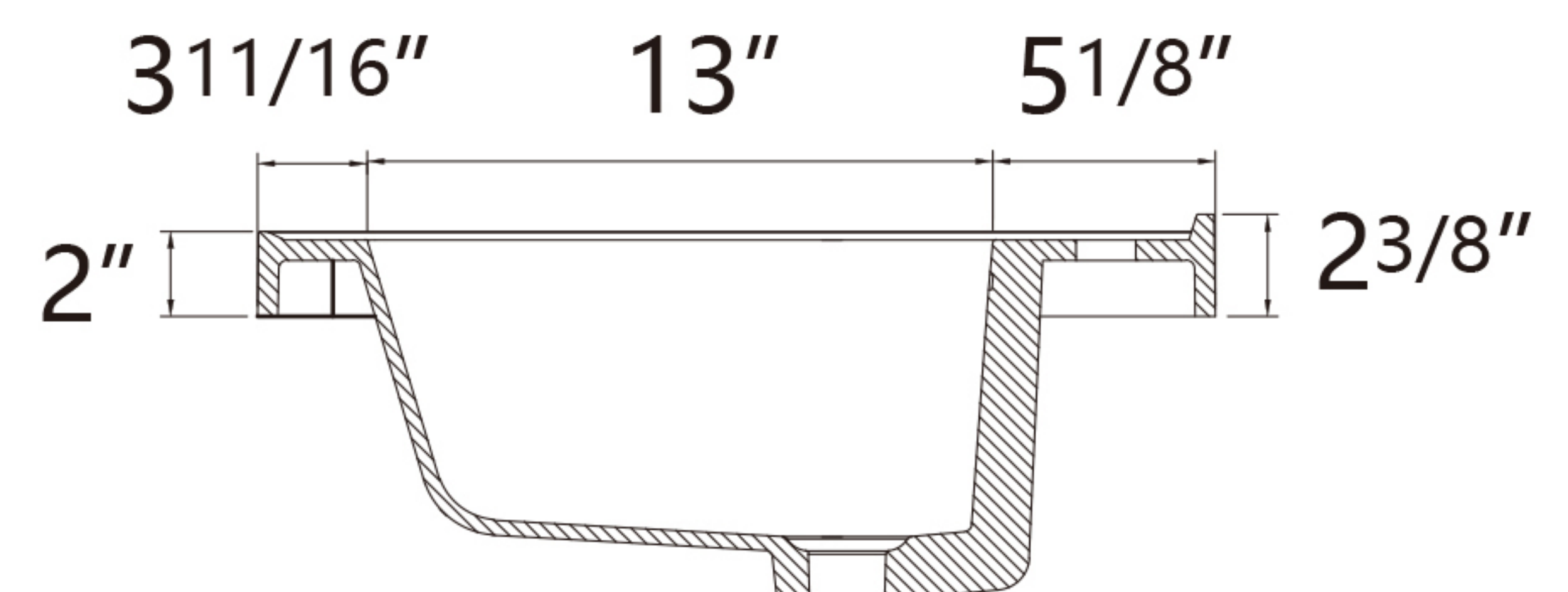
Side View
