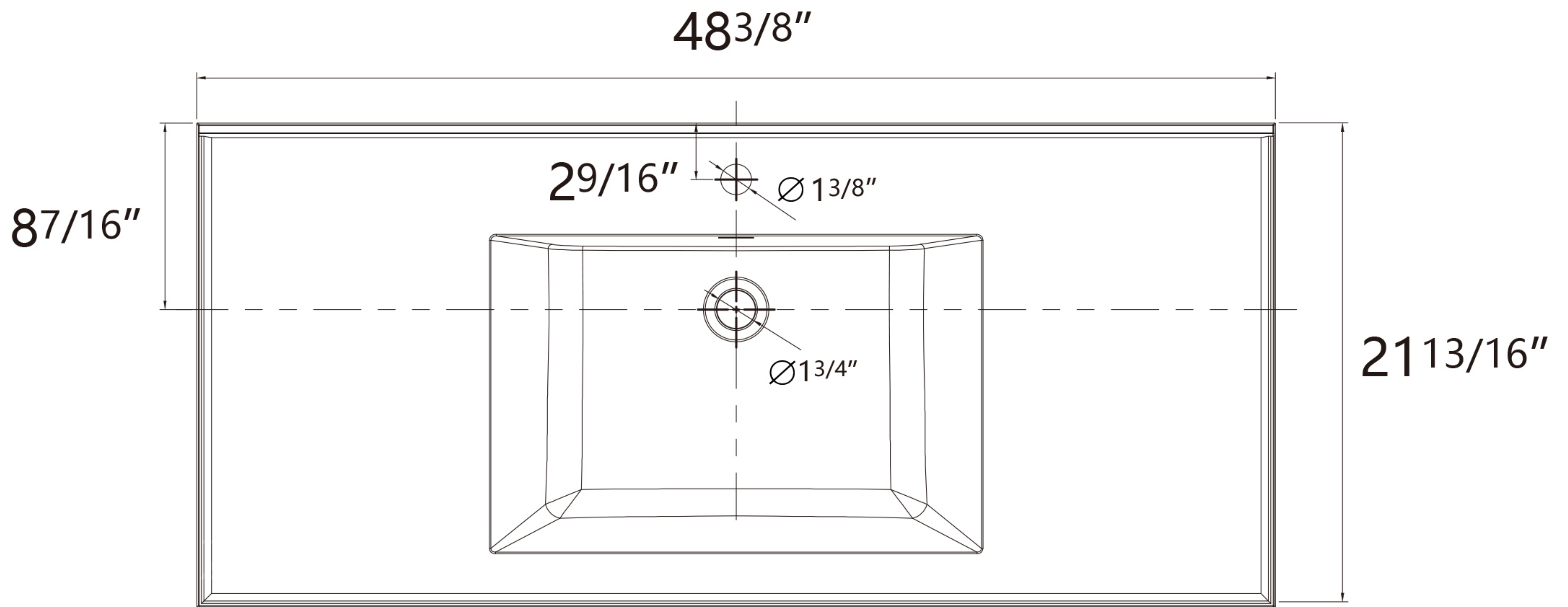
Top View
