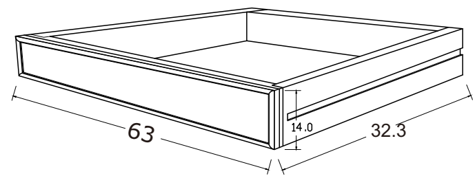
DRAWER DETAIL
