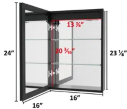
Cabinet Dimensions
