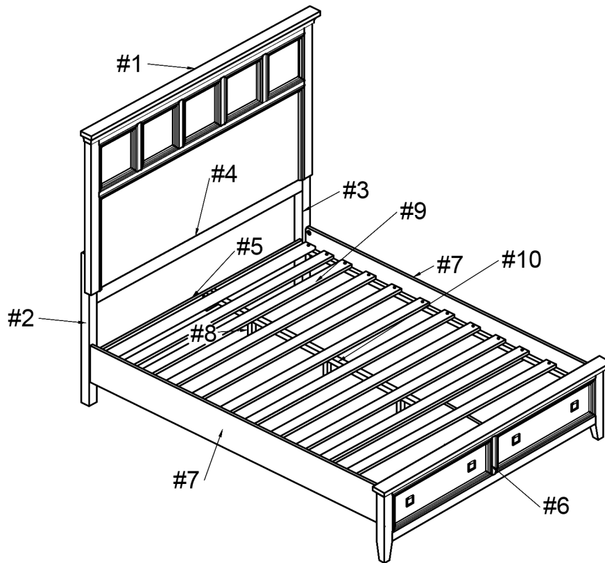
Exploded View
