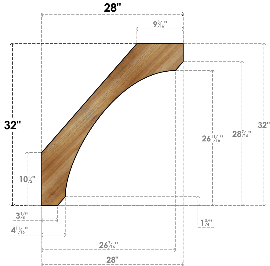
SIDE
