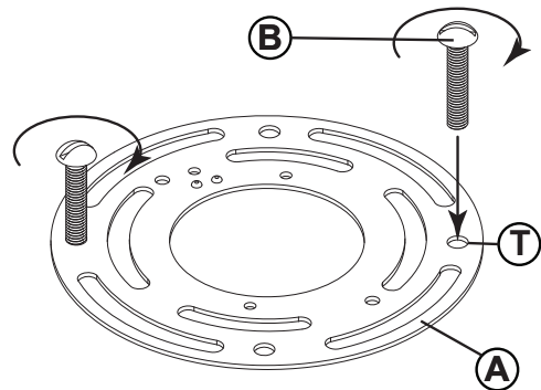
DRAWING 1 - MOUNTING
