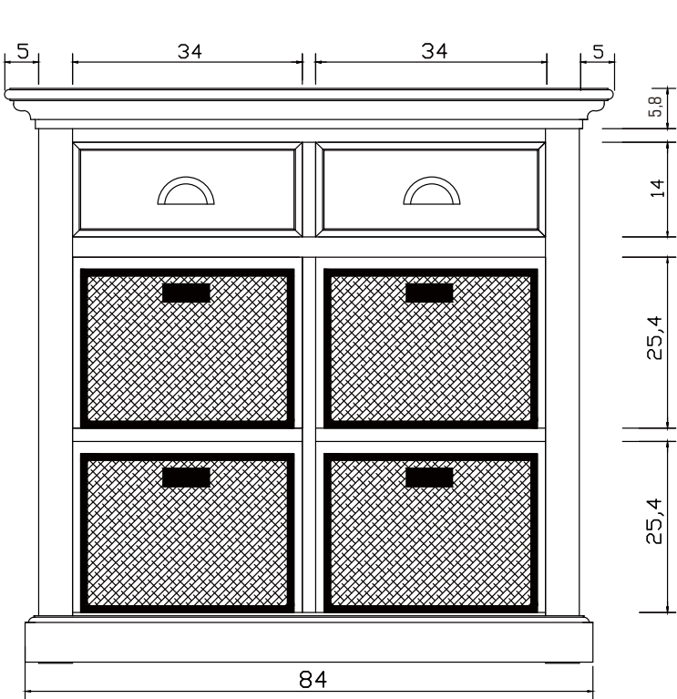
FRONT VIEW
