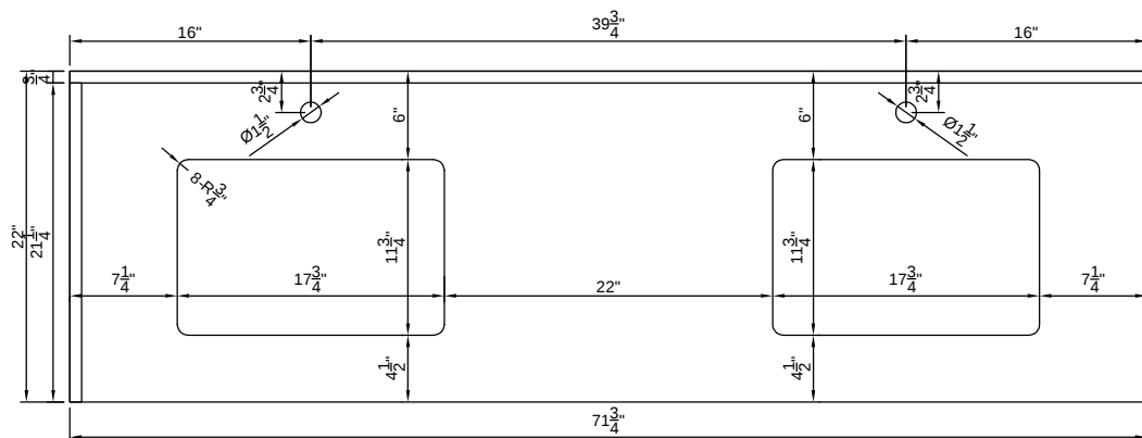
TOP VIEW OF VANITY CABINET
