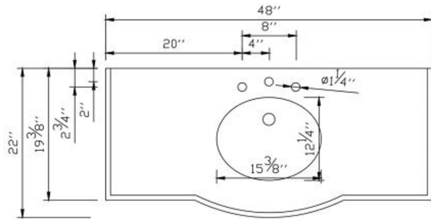
TOP VIEW
