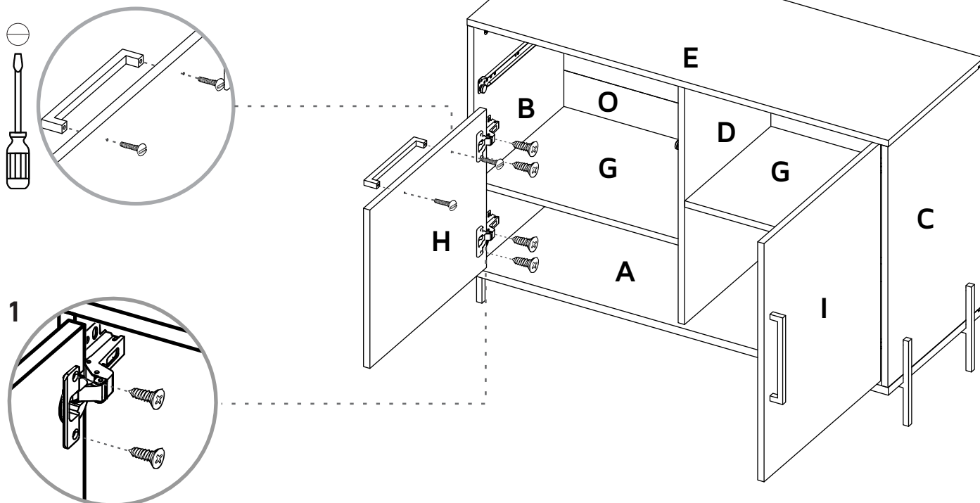
Hinge adjustment
