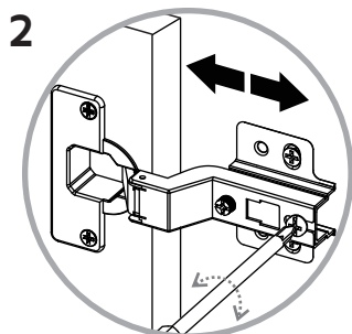
Depth adjustment
