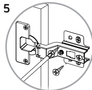
Secure Hinge
