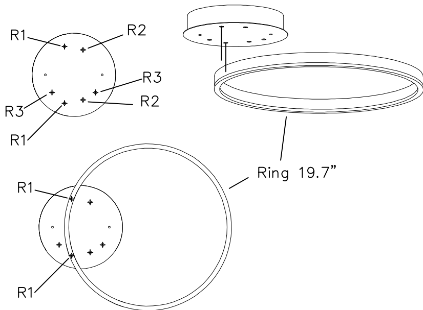
1. Assemble R1 (first Layer)
