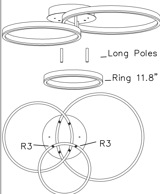
3. Assemble R3 (3rd Layer)
