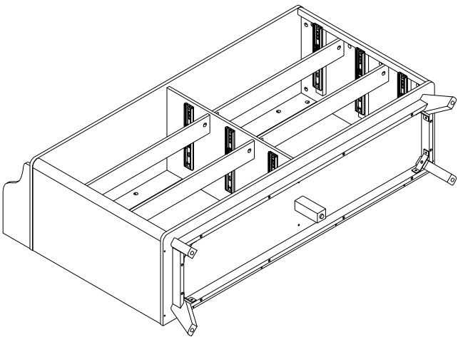
Completed Assembly
