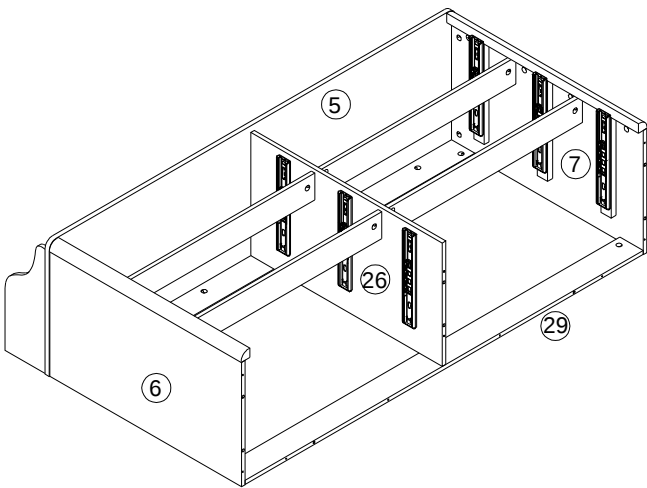
Completed Assembly
