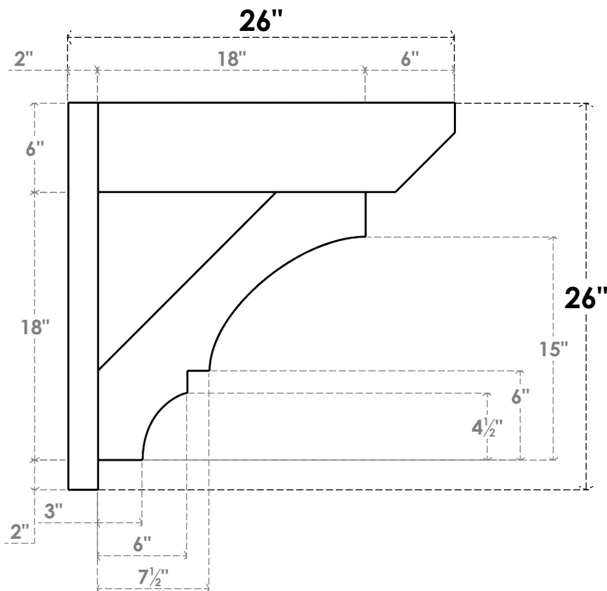
SIDE PROFILE
