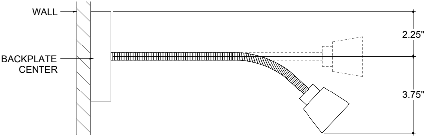
SIDE VIEW
