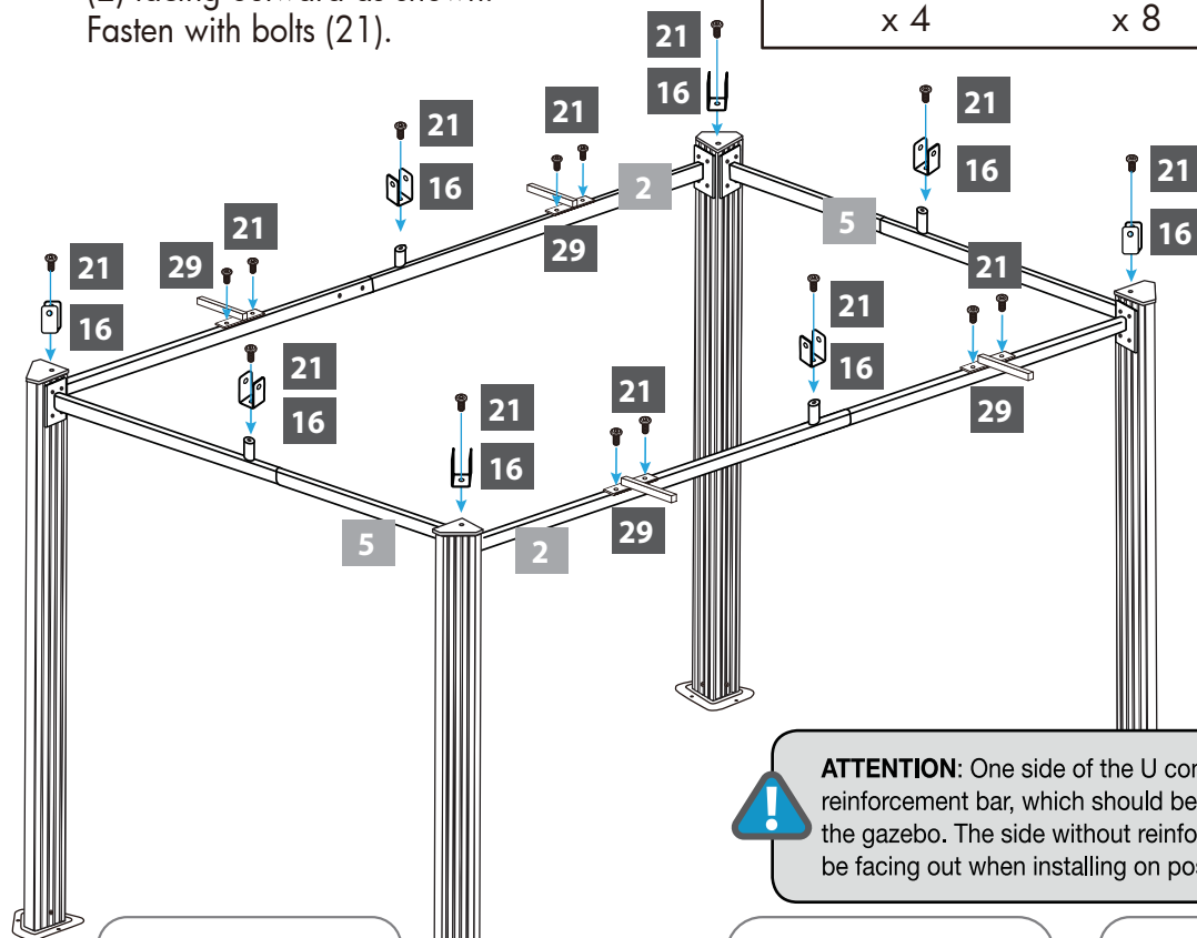
Canopy Support (29) x 4
