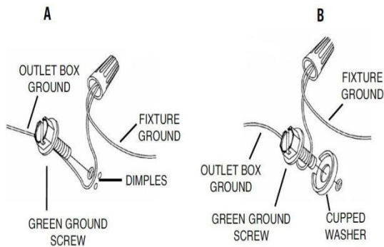
Ground line(if have) connection
