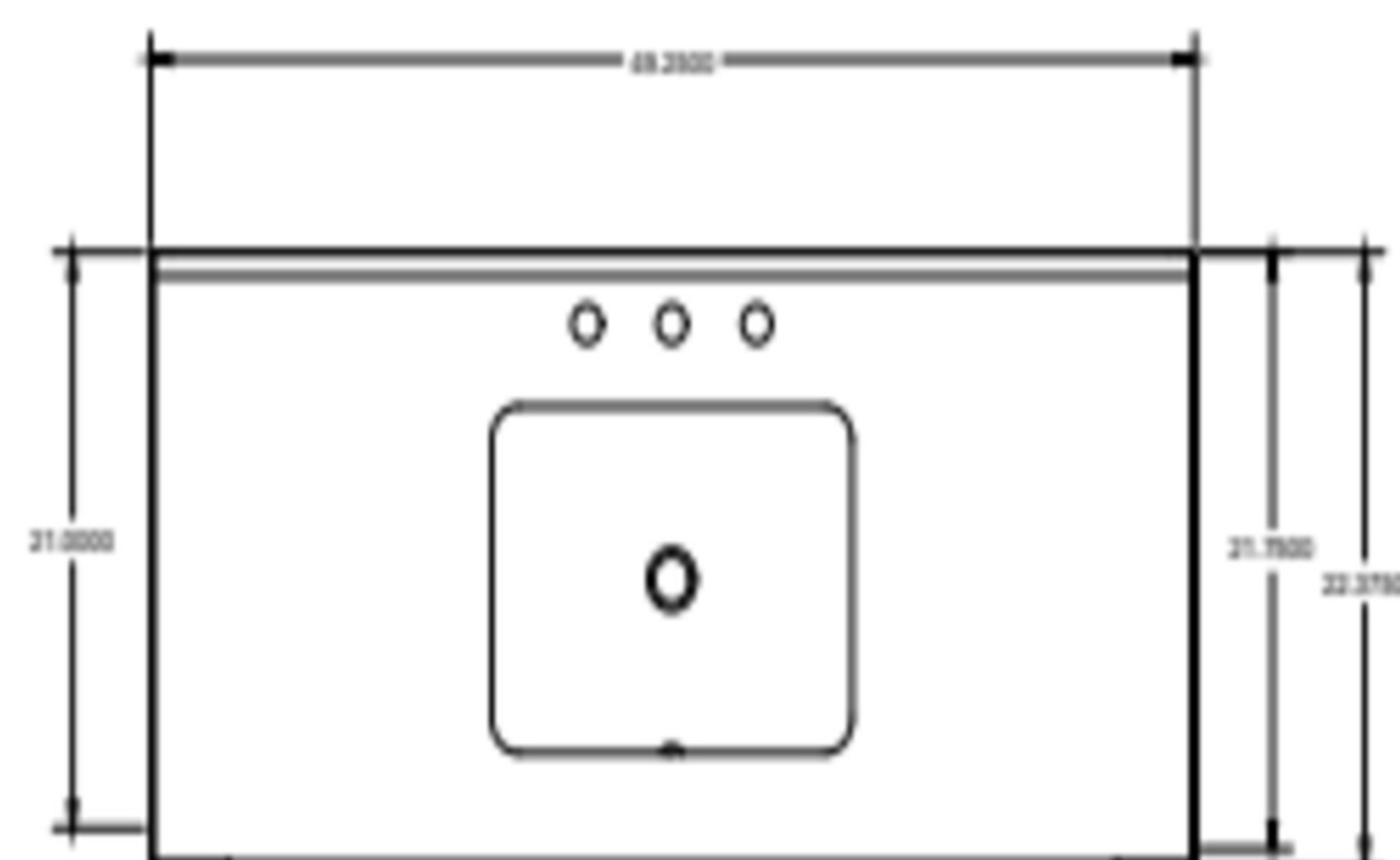
TOP VIEW
