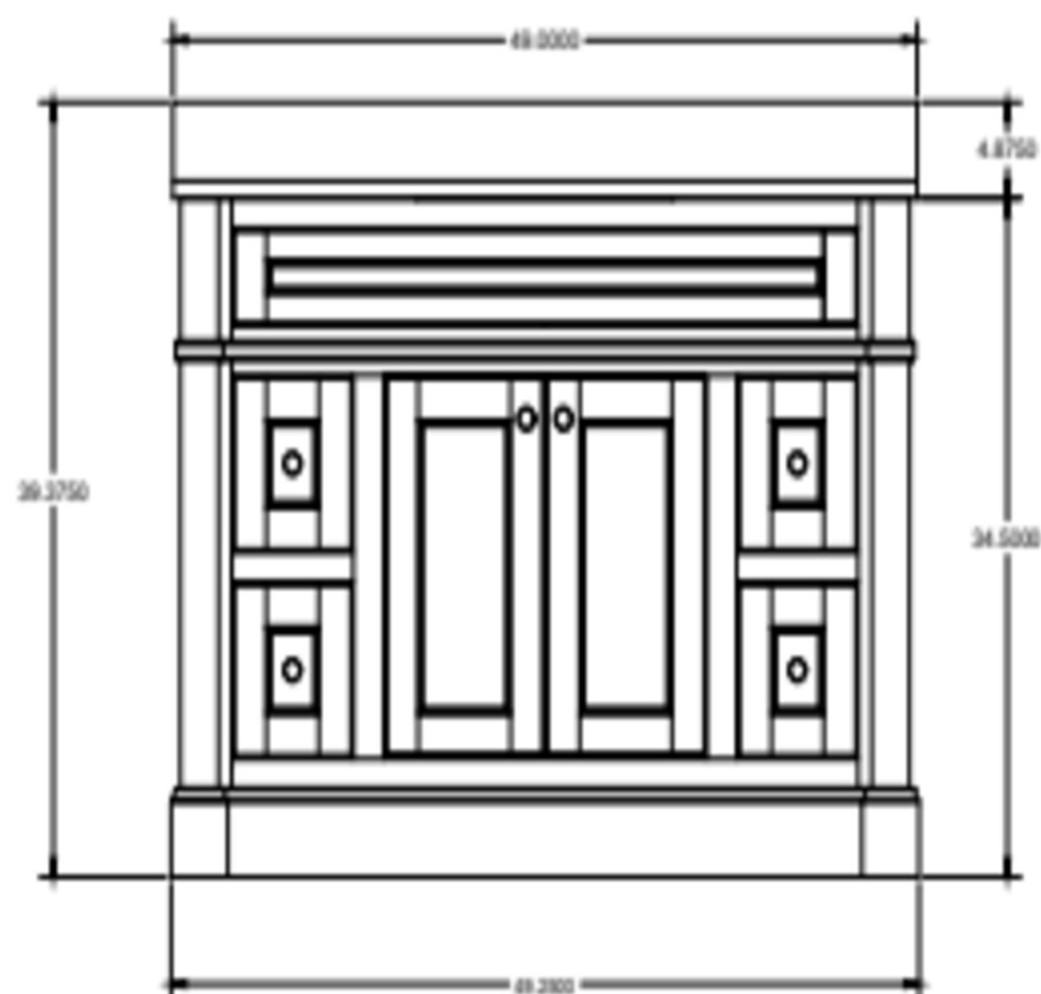
FRONT VIEW
