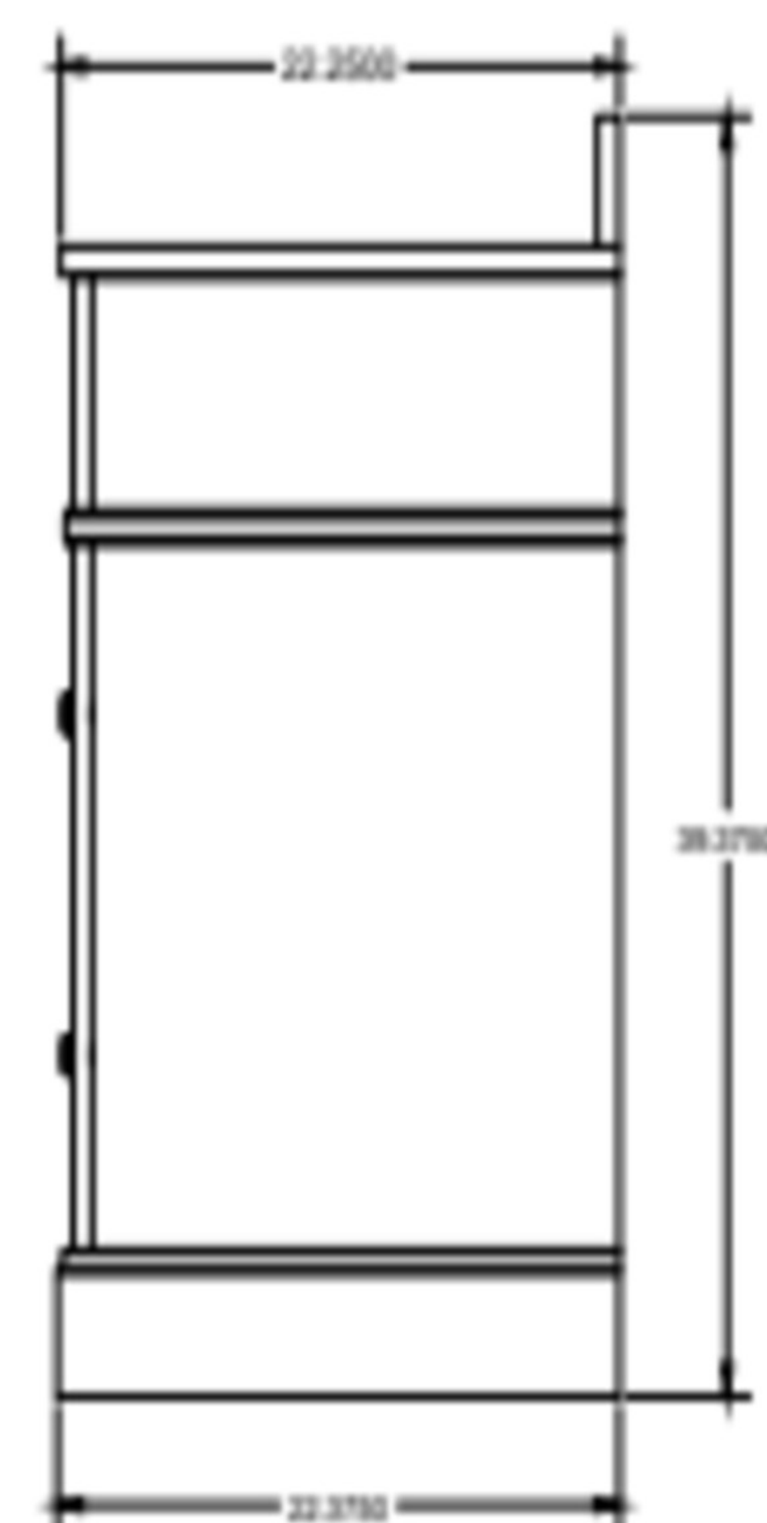
SIDE VIEW
