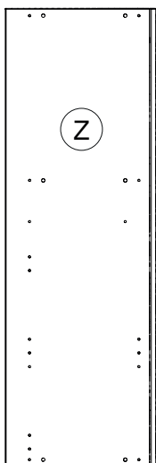
FI8995 1061x353x30mm
