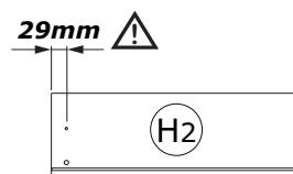
CS3766 473x157x16mm
