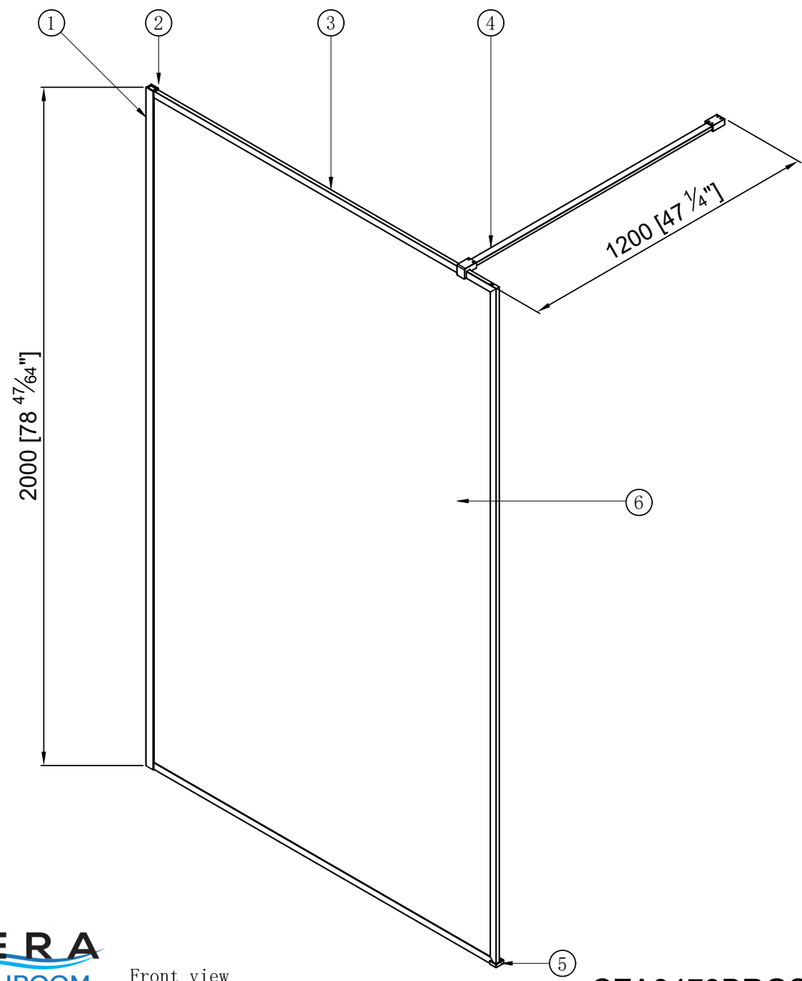
Front view
