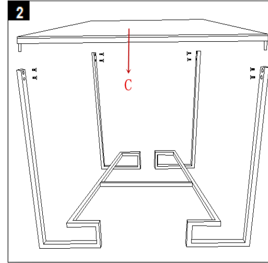
Step 2 Assemble the Top shelf (C) to side legs (A) together using 8 screws (E).
