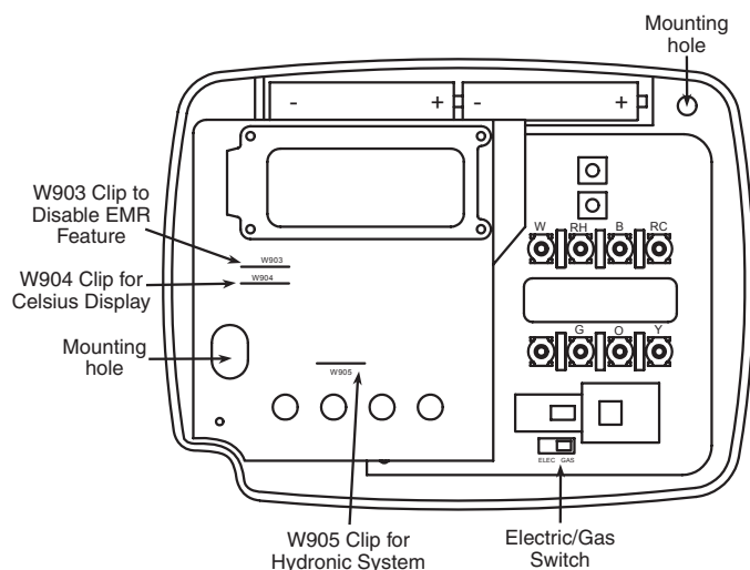
Figure 1. Thermostat base
