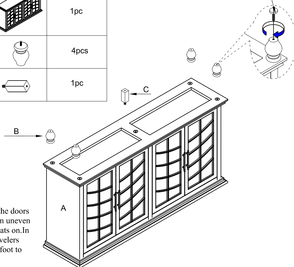
Adjustable leveler
