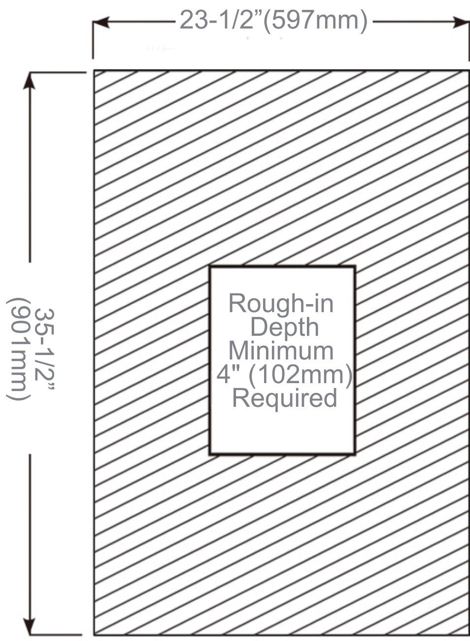
Rough-in Dimensions
