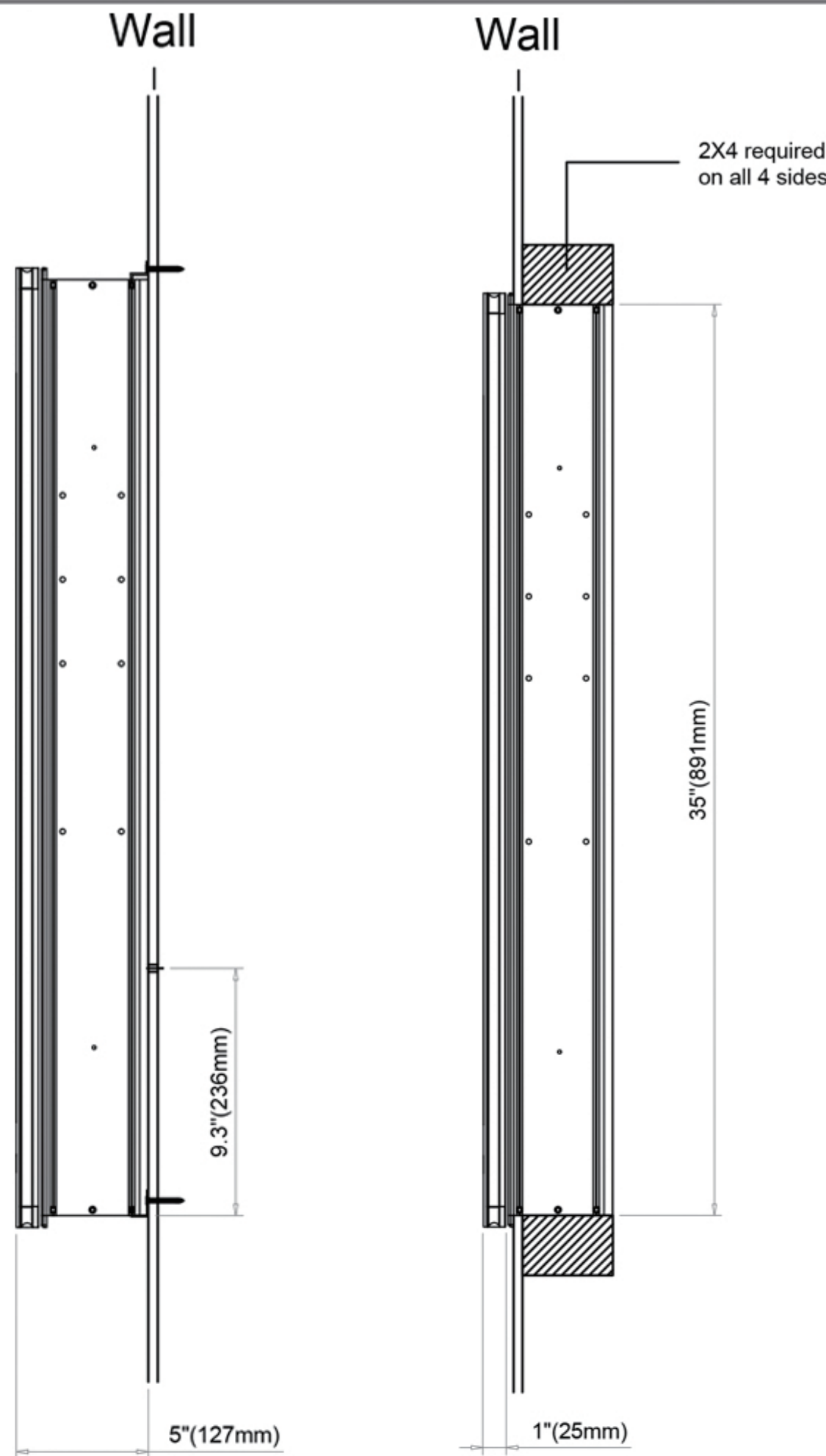
Surface Mount
