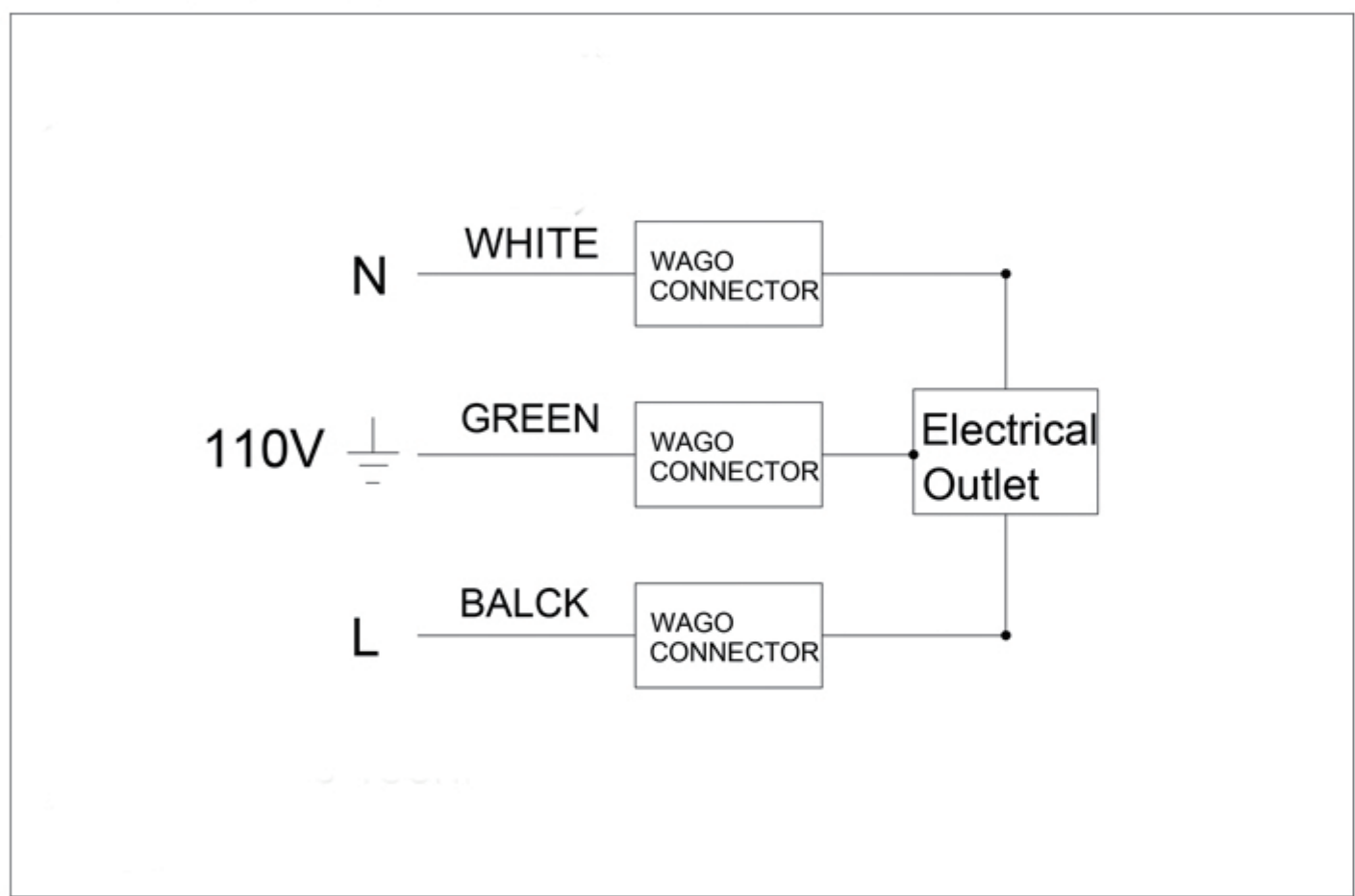
Circuit Diagram
