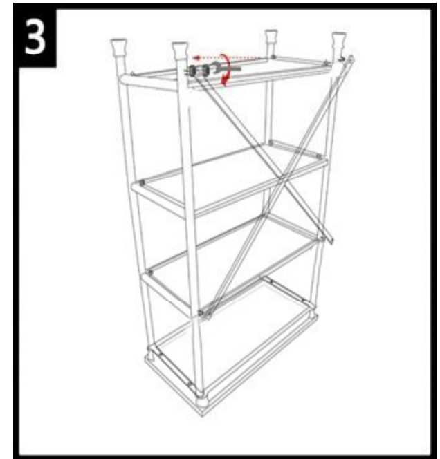
Step 3 Screw the Easels(E) into the legs(B) with 2 hexagon screw
