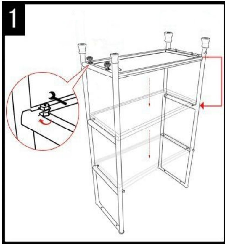
Step 1 Screw the Shelves(C ) into the Legs(B)
