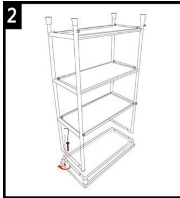
Step 2 Screw the Legs(B) into Top(A)
