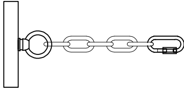
Canopy and hanging chain 1PCS
