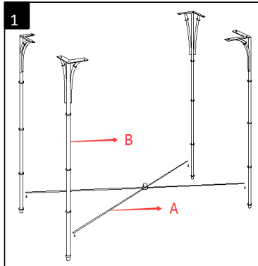
Step 1 Assemble the Legs(B) Stretcher(A) together using 4 Screws.
