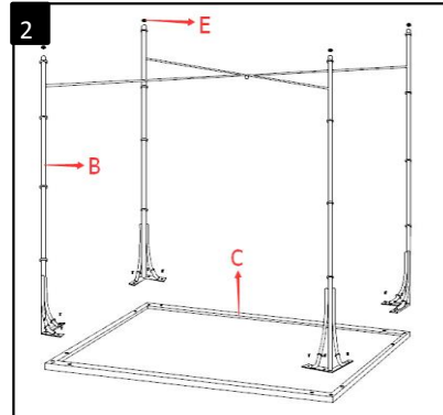
Step 2 Assemble the Legs(B) Top Frame(C) Felt pad(E) together using 12 Screws.
