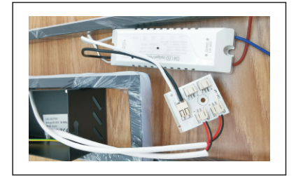
4.Any pair of lamp power cables are plugged into the driver.On the board, ignore the extra sockets.
