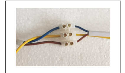
6.Input drive power cord and household power cord.Dock with the terminal blocks, and then lock the screws.
