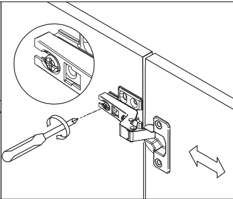
C. Front-to-Back by slacking the hinge arm mounting screw
