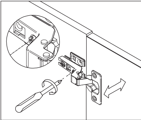
B. Lateral adjustment by screw adjusting
