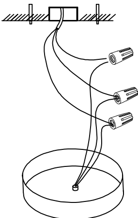
3. Connect wires
