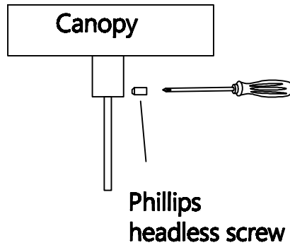
2. Height adjustment -use screwdriver to turn Phillips headless screw in a clockwise direction until snug.
