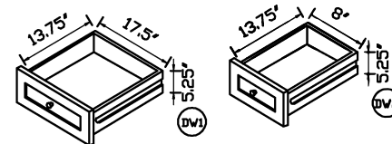
Drawer Interior Size
