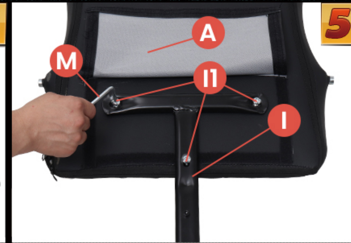
Assemble the Back plate. The side with the protrusion is the outside.
