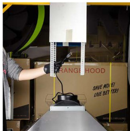
18. Connect the duct to the damper/air flapper onto the main unit.
