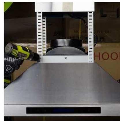
20. Feed the power cord through the ceiling hole.
