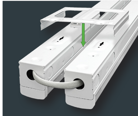
Brackets snap into place for tandem mounting
