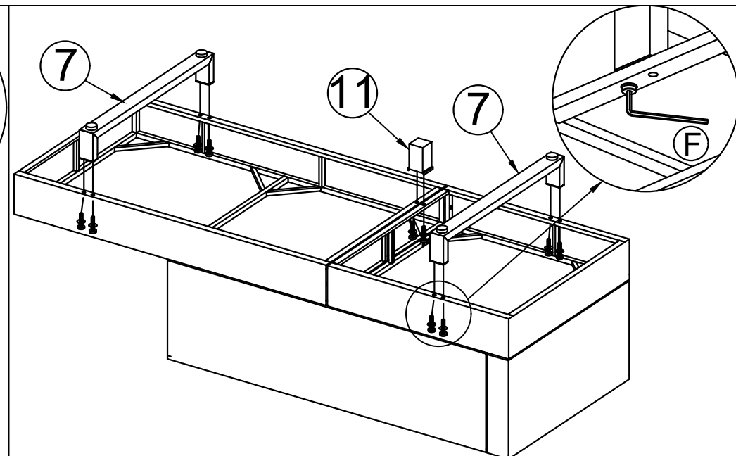
Step 8: Connect The Part from Step 7 & Leg Sofa Frame (7), Leg Middle Bench Frame (11) tighten Bolt (C), Flat Washer (E) with Allen Key (F).
