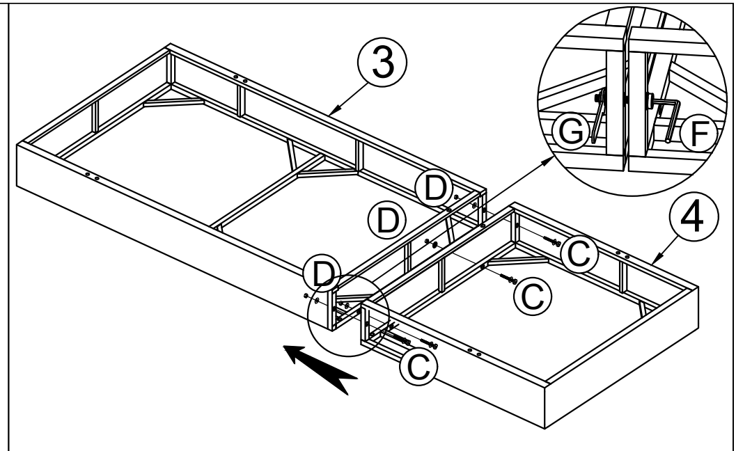
Step 4: Connect Right Bench Frame (3) & Corner Bench Frame (4), tighten Bolt (C), Flat Washer (E) & Nut (D) with Allen Key (F), Key (G).
