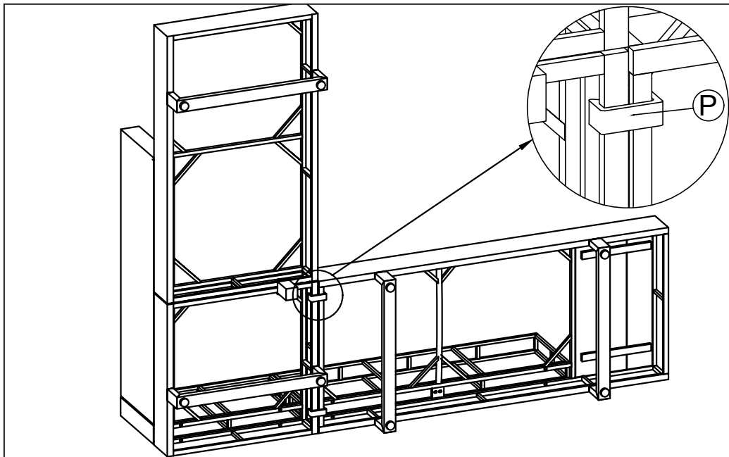
Step 10: Connect Left Bench & Right Bench with Connector (P).
