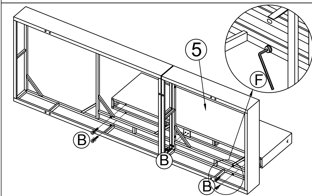
Step 5: Connect The Part from Step 4 & Back Bench Frame (5), tighten Bolt (B), Flat Washer (E) with Allen Key (F).
