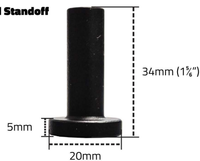
NT.1303-34mm.08 (For doors up to 1 1/2" thick)
