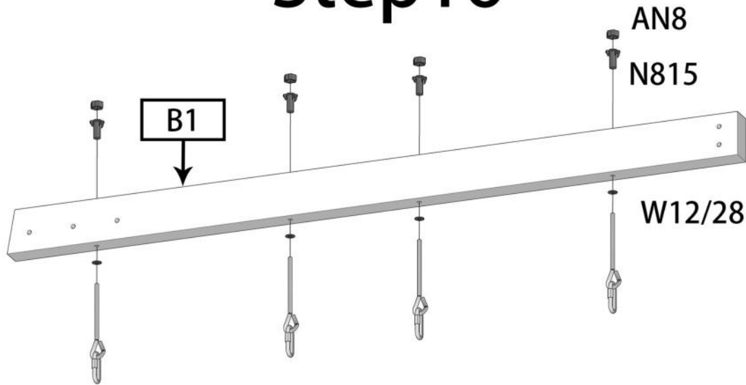
SWING HANGER-129006
