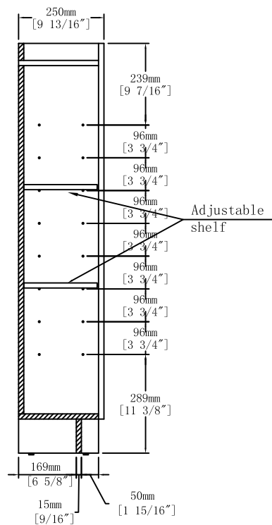
Side View
