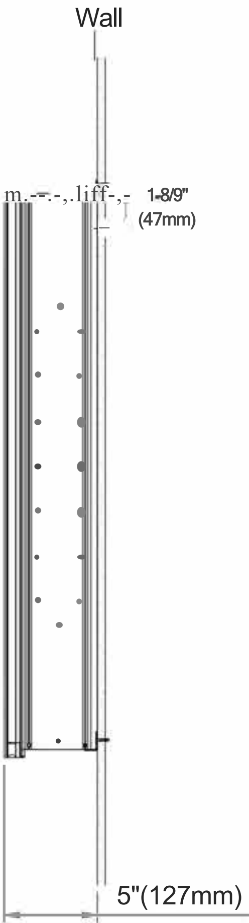
Surface Mount
