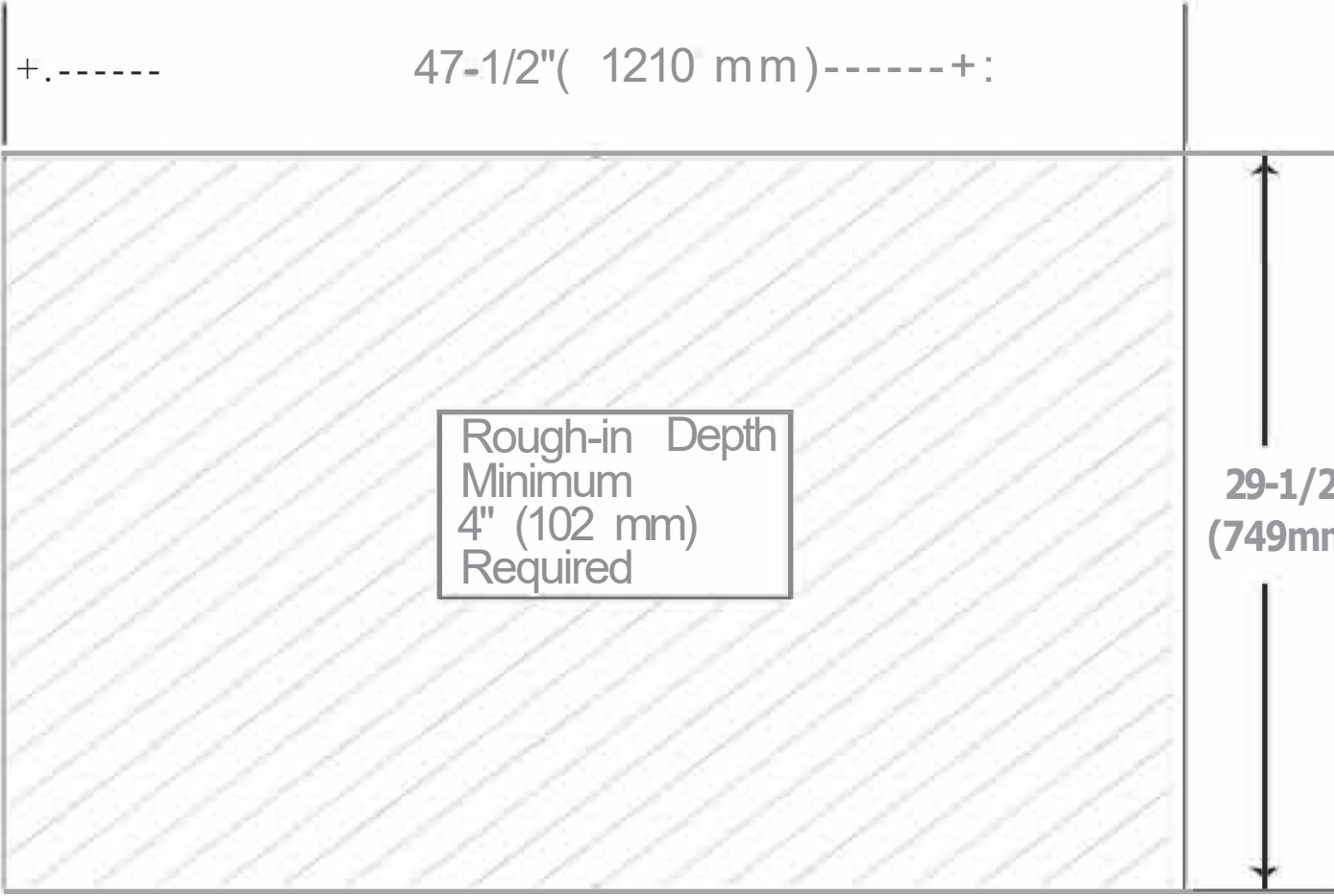
Rough-in Dimensions
