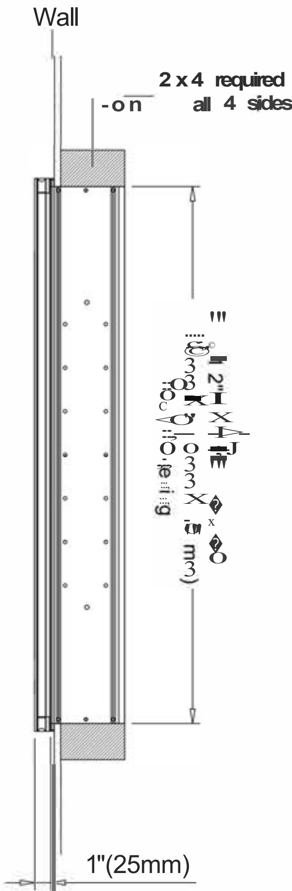
Recessed Mount
