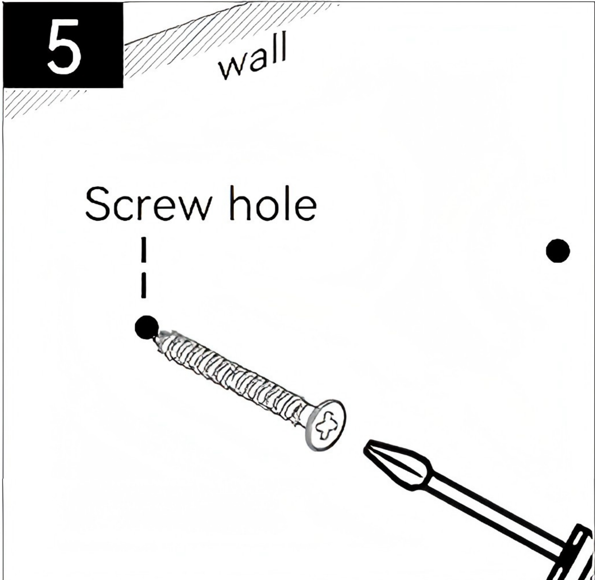
Screw in the tapping screw with a screwdriver.
