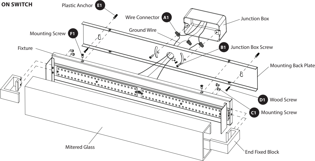
FIG. 2 MOUNT ON JUNCTION BOX
