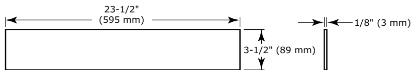
Wooden Insert Dimensions
