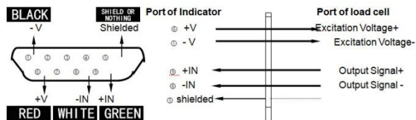
(Graph 2-3) Drawing of connecting of load cell
