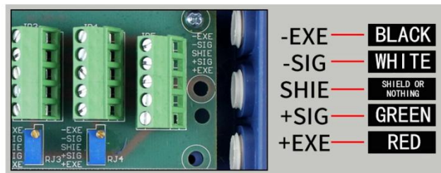
(Graph 2-3) Drawing of connecting of load cell
